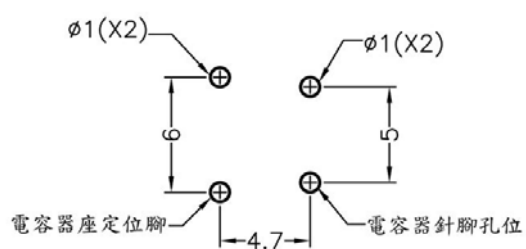
MOUNTING HOLE
