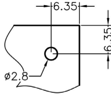
MOUNTING HOLE
