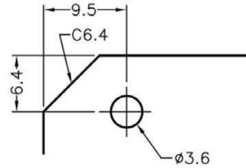
MOUNTING HOLE
