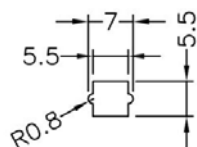
CHASSIS MOUNTING HOLE THICKNESS:0.8~1.2
