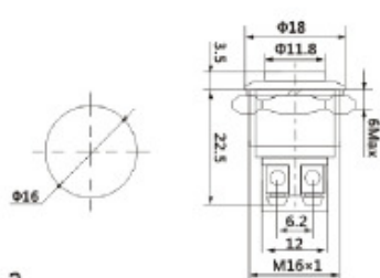
GQ-16H-2 3A 250VAC ; 2A 36VDC
