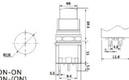
DS-612C ON-ON DS-613C ON-(ON) 2A 250VAC;5A 125VAC
