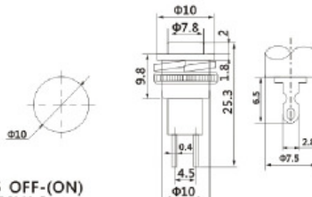
DS-314 OFF-(ON) DS-315 ON-(OFF) 0.5A 250VAC
