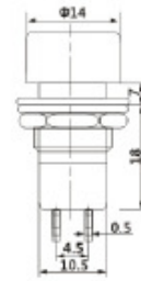
PBS-16A ON-OFF PBS-16B OFF-(ON) 1A 250VAC
