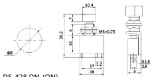
DS-428 ON-(ON) 5A 250VAC
