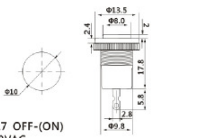
DS-211 ON-OFF DS-213 OFF-(ON) 1A 250VAC
