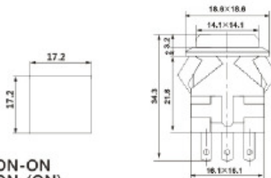
KD2-21 ON-ON KD2-22 ON-(ON) 3A 250VAC; 6A 125VAC (With LED)
