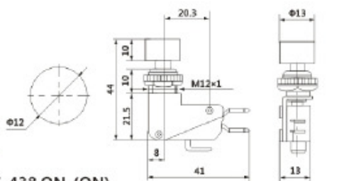
DS-438 ON-(ON) 16A 250V/AC
