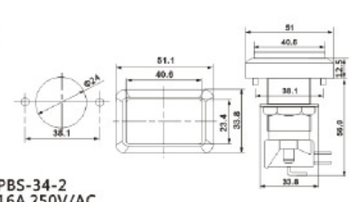
PBS-34 16A 250V/AC
