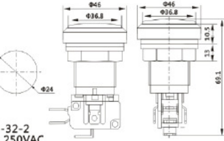
PBS-32 16A 250VAC
