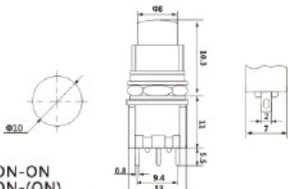
DS-622 ON-ON DS-623 ON-(ON) 2A 250VAC;5A 125VAC
