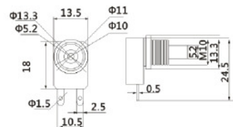
PBS-104 ON-OFF 1A 250VAC
