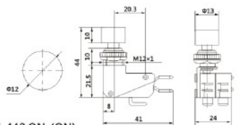
DS-448 ON-(ON) 16A 250V/AC
