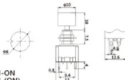
DS-612 ON-ON DS-613 ON-(ON) 2A 250VAC;5A 125VAC
