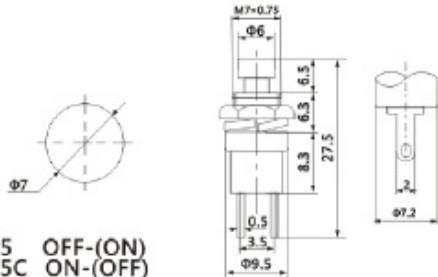
KAX-3 OFF-(ON) 0.5A 250VAC
