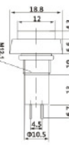
PBS-13A ON-OFF PBS-13B OFF-(ON) 1A 250VAC
