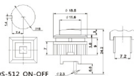
DS-512 ON-OFF DS-513 OFF-(ON) 1A 250VAC
