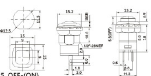
DS-225 OFF-(ON) DS-226 ON-OFF 1A 250VAC
