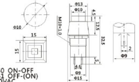
DS-450 ON-OFF DS-451 OFF-(ON) 1A 250VAC
