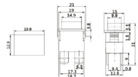
PS23-16 ON-OFF 16A 250VAC
