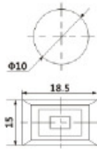
DS-470 ON-OFF DS-471 OFF-(ON) 1A 250VAC
