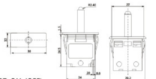
PBS-37 ON-(OFF) 1A 125VAC ; 0.5A 250VAC
