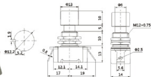
PBS-24A-3 ON-OFF 6A 250VAC;10A 125VAC
