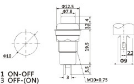
R13-502 OFF-(ON) 1A 250VAC
