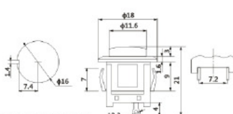
DS-510K ON-OFF DS-511K OFF-(ON) 1A 250VAC
