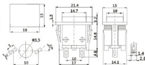
PBS-30B OFF-(ON) 1A 250VAC;3A 125VAC
