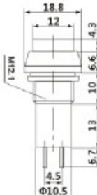
PBS-14A ON-OFF PBS-14B OFF-(ON) 1A 250VAC
