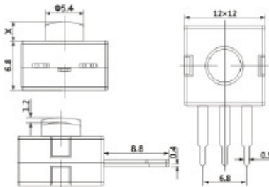
PBS-05 ON-ON-OFF 1A 30VDC
