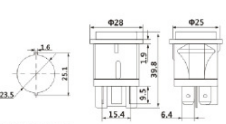
PS18-16 ON-OFF 16A 250VAC
