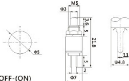
DS-101 OFF-(ON) 0.5A 125VAC
