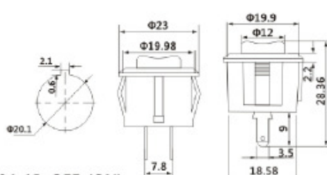
PS04-1R OFF-(ON) 1A 250VAC
