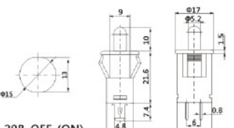
PBS-29B OFF-(ON) 3A 250VAC
