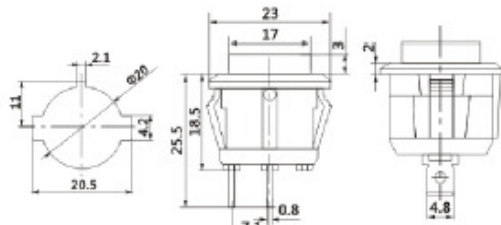
DS-858 OFF-(ON) 6A 250VAC;10A 125VAC
