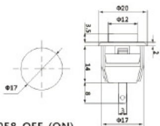
DS-058 OFF-(ON) 1A 250VAC
