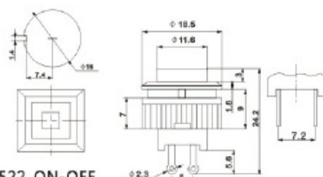
DS-522 ON-OFF DS-523 OFF-(ON) 1A 250VAC(With LED)
