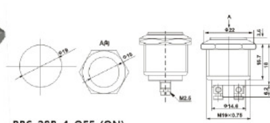
PBS-28B-4 OFF-(ON) 6A 125V/AC 3A 250V/AC
