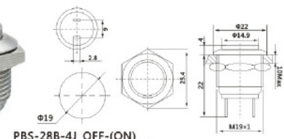
PBS-28B-4J OFF-(ON) 6A 125V/AC 3A 250V/AC
