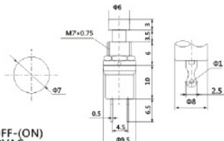
DS-402 OFF-(ON) 0.5A 125VAC
