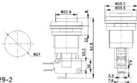
PBS-29-2 16A 250VAC
