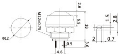
PBS-33B OFF-(ON) 1A 250VAC
