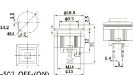
DS-502 OFF-(ON) DS-503 ON-(OFF) 1A 250VAC
