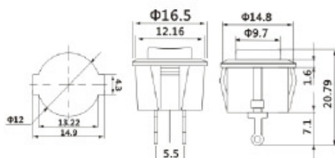
PS14-1R OFF-(ON) 1A 250VAC
