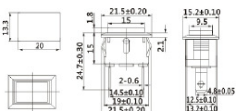
PBS-101 OFF-(ON) 6A 250VAC;10A 125VAC
