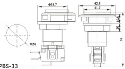
PBS-33 16A 250V/AC
