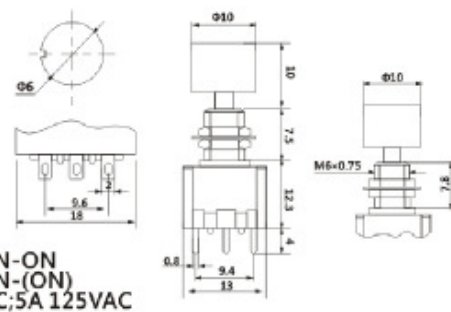
DS-622C ON-ON DS-623C ON-(ON) 2A 250VAC;5A 125VAC
