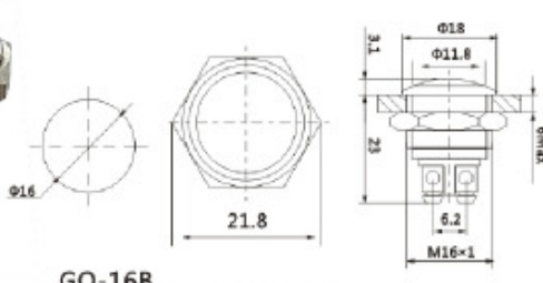
GQ-16B 3A 250VAC ; 2A 36VDC
