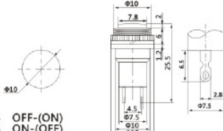
PBS-105 OFF-(ON) PBS-105C ON-(OFF) 0.5A 250VAC
