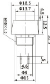
DS-470 ON-OFF DS-471 OFF-(ON) 1A 250VAC
