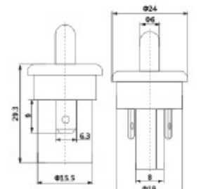
PBS-35B OFF-(ON) 3A 125VAC ; 1A 250VAC
