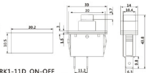
RK1-11D ON-OFF 15A 250VAC;20A 125VAC
