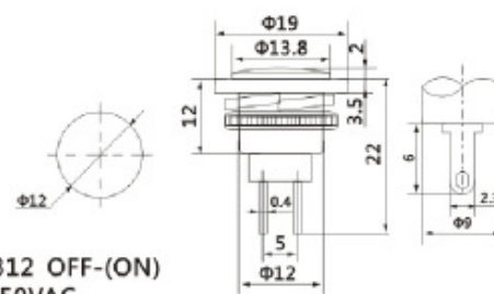
DS-324 OFF-(ON) 1A 250VAC
