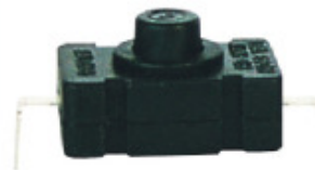
PBS-01A ON-OFF 1A 250VAC; 1A 30VDC
