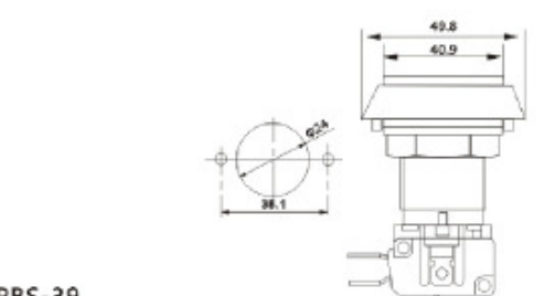
PBS-39 16A 250V/AC
