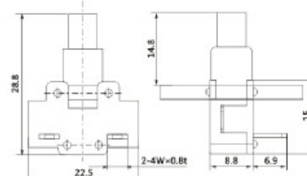
PBS-19 10A 125VAC ; 6A 250VAC
