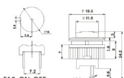
DS-510 ON-OFF DS-511 OFF-(ON) 1A 250VAC
