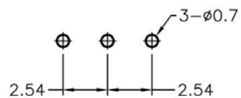
MOUNTING HOLES
