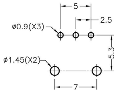
MOUNTING HOLES
