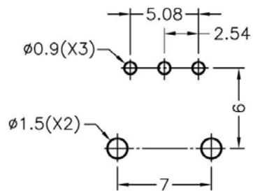
MOUNTING HOLES
