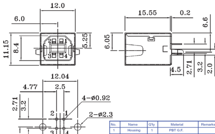
(COMPONENT SIDE) PCB LAYOUT
