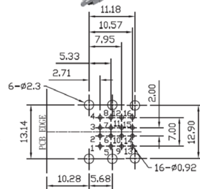
BOTTOM VIEW RECOMMENDED PCB LAYOUT
